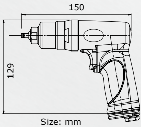
22106 1/4" Air Impact Wrench
