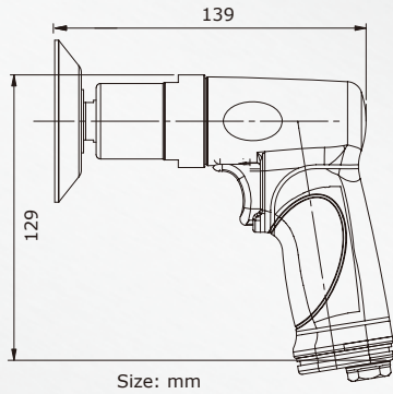
50006 Pistol Polisher
