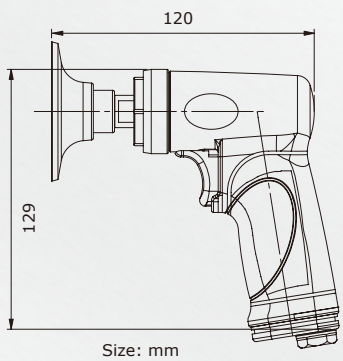
54106 3" Disc Sander
