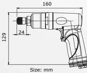
62106 1/4" Air Screwdriver
