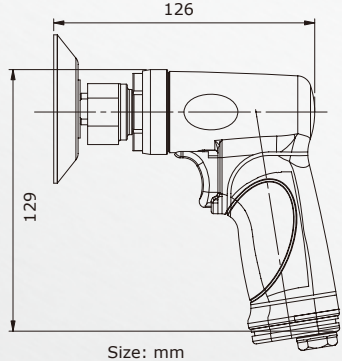
51406 Orbital Sander (3 mm Orbit)
