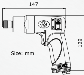
64206 1/4" Air Screwdriver (Direct Drive)
