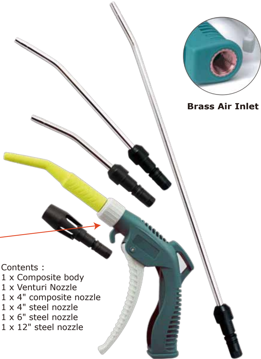
A216M-6K Air Blow Gun Kit
